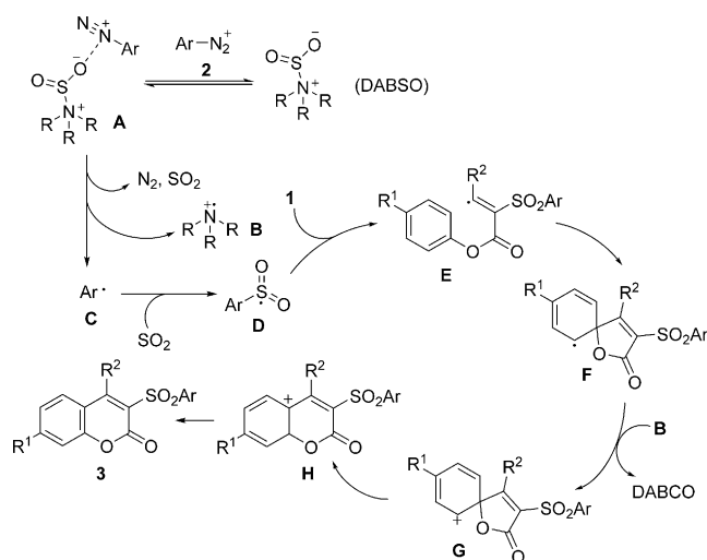
Scheme 4. Proposed mechanism.
